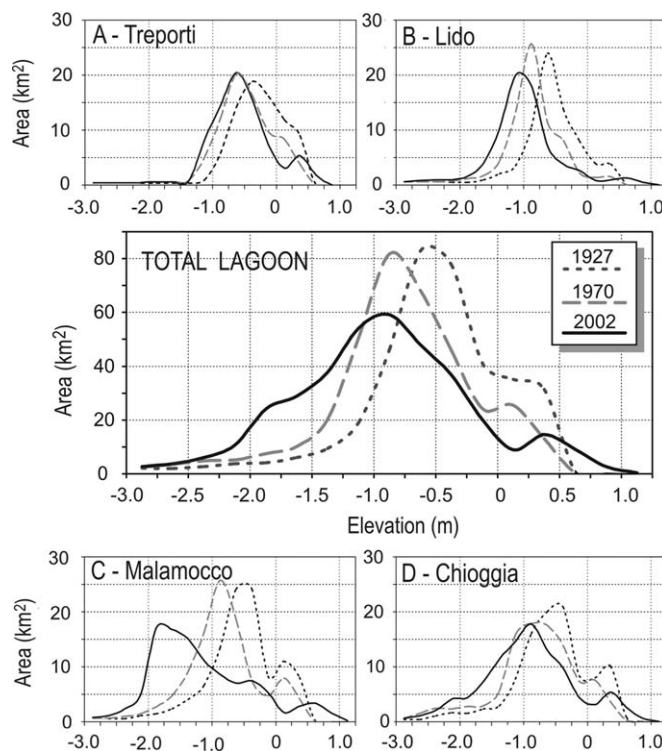
Fig. 4. The Distribution of surface areas of specific elevation categories in 1927 (dotted line), 1970 (dashed line) and 2002 (solid line) in whole Lagoon of Venice (central plot) and sub-basins A–D.
